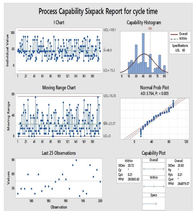
Figure 5 Process Capability Sixpack Report for cycle time
